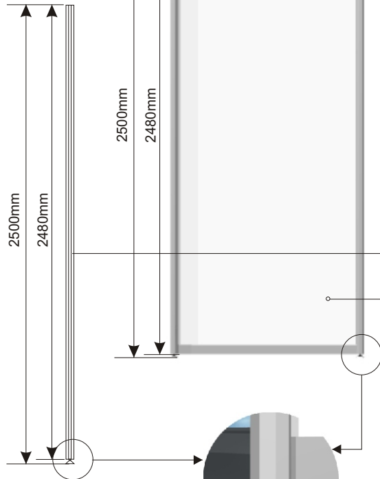
ADJUSTABLE FOOT
